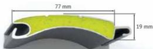
Lame Isolante 77 mm Shutter Slats with isolation 77 mm
